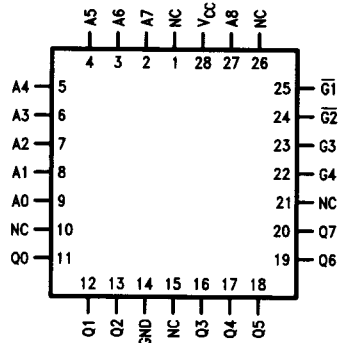
Plastic Leaded Chip Carrier (PLCC)
