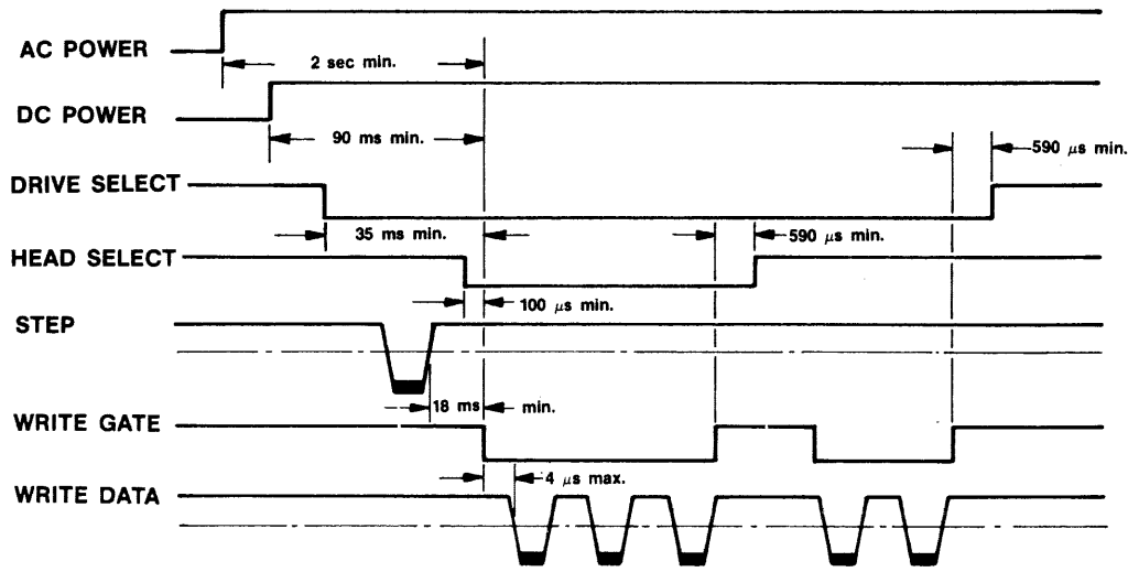
Write Timing
