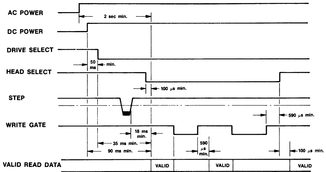
Read Timing
