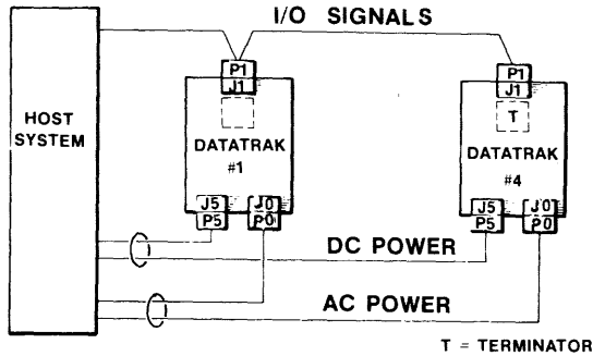
Interface Connection
