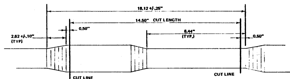
CABLE DETAIL
