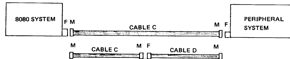
INTER CHASSIS CONNECTOR DETAIL
