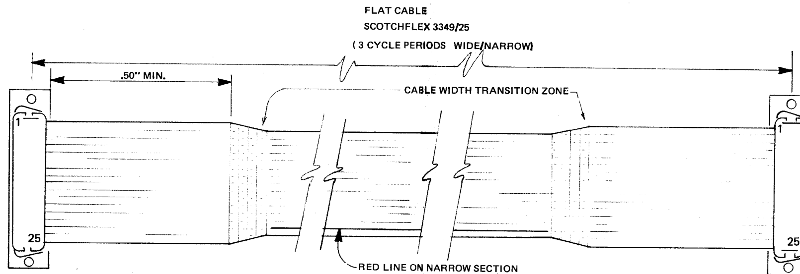
INTER CHASSIS CONNECTOR DETAIL
