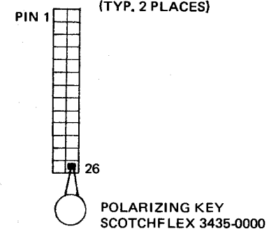
26 PIN SOCKET CONNECTOR DETAIL (TYP. 2 PLACES)
