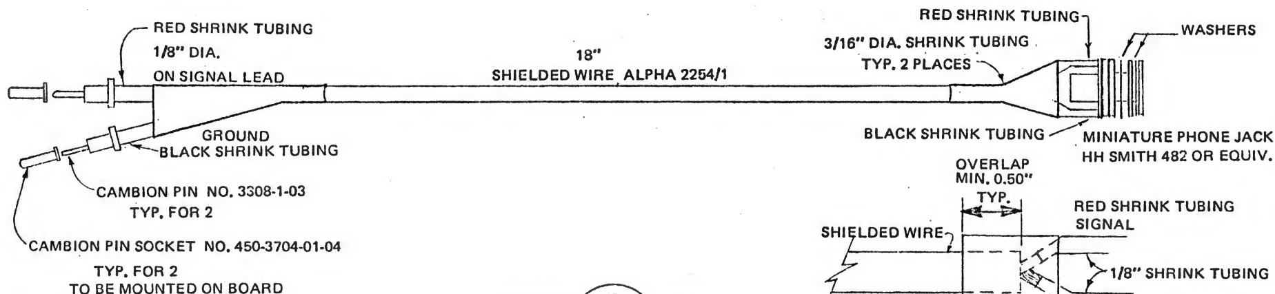
PHONE JACK SECTION TUBING DETAIL
