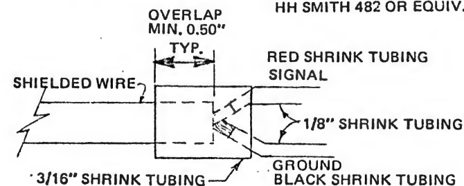
PHONE JACK SECTION TUBING DETAIL
